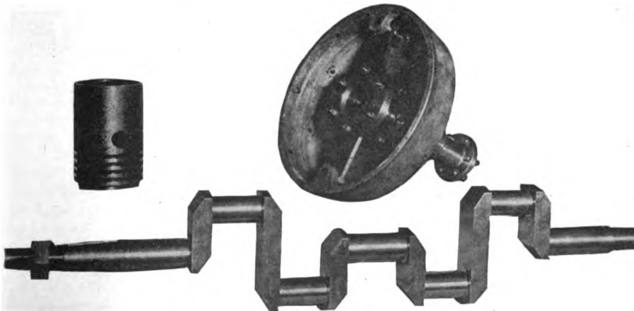
ALUMINUM CLUTCH, LONG PISTON AND FOUR-THROW CRANKSHAFT OF SIMPLEX CAR.
